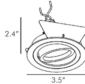
Overall Dimensions
